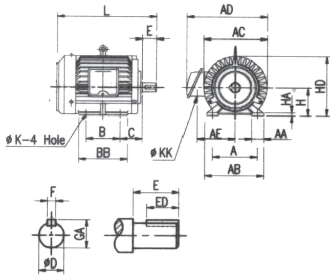
FOOT MOUNTED TYPE (HORIZONTAL TYPE)
